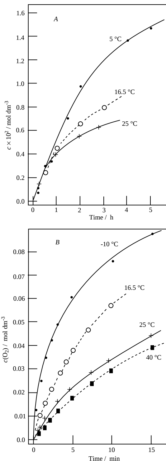
Figure 1. Accumulation of cyclohexanol and cyclohexanone (total concentration, c ) in cyclohexane ( 0.46 \text{ mol dm}^{-3} ) oxidation with \text{H}_2\text{O}_2 ( 0.6 \text{ mol dm}^{-3} ) catalyzed by Mn(IV)-compound 2 catalyst (1.0 mg; volume of the reaction solution 1 mL) in the presence of acetic acid ( 0.25 \text{ mol dm}^{-3} ) at various temperatures (graph A) and oxygen evolution by the same system [in the absence of cyclohexane; Mn(IV)-compound 2 catalyst, 1.5 mg; volume of the reaction solution 2.5 mL] at various temperatures (graph B).
